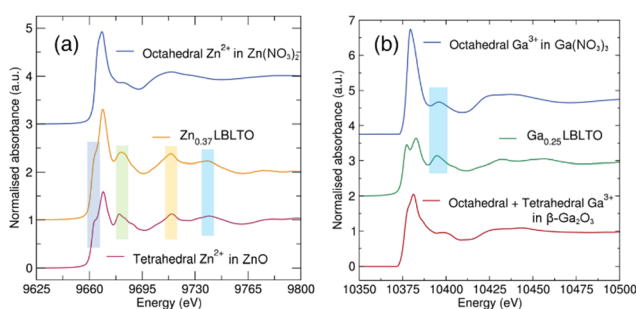
Fig. 4 (a) XANES region of the XAS data measured on the Zn K-edge for Li_{5.25}Zn_{0.37}BaLa_2Ta_2O_{12} , and Zn(NO_3)_2 \cdot 6H_2O and ZnO standards. (b) XANES region of the XAS data measured on the Ga K-edge for Li_{5.25}Ga_{0.25}BaLa_2Ta_2O_{12} and Ga(NO_3)_3 \cdot 9H_2O and \beta - Ga_2O_3 standards. Coloured boxes indicate common features in the XANES profiles between the different materials analysed.
