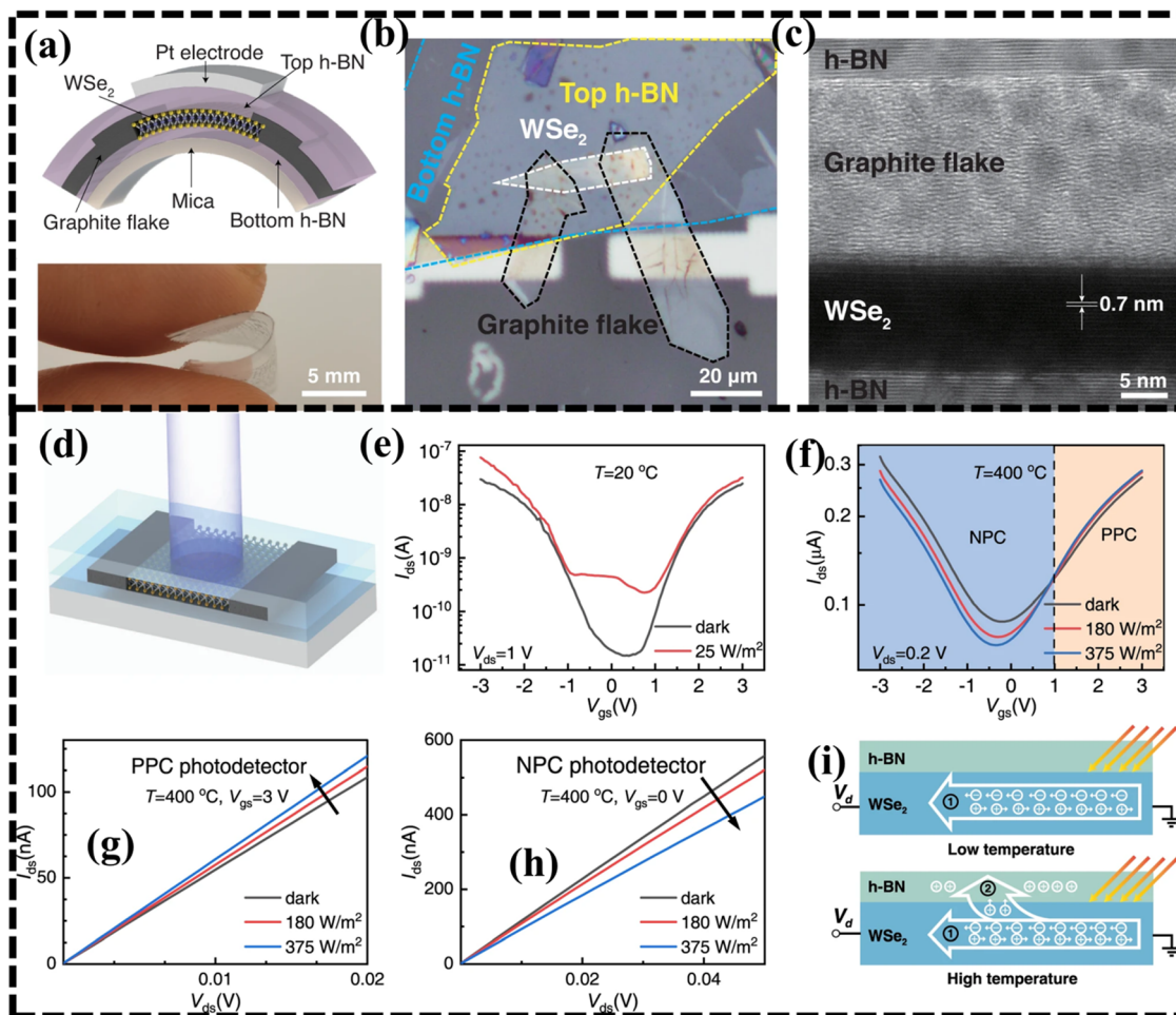
Fig. 5 (a) Schematic view of the \text{WSe}_2 photodetector with h-BN encapsulation and graphite electrodes. (b) Optical image of the device. (c) HR-TEM cross-sectional image of the device. (d) \text{WSe}_2 photodetector under illumination. (e) I_{\text{ds}}-V_{\text{gs}} characteristics under dark and illumination at 20^\circ\text{C} . (f) I_{\text{ds}}-V_{\text{gs}} characteristics under dark and illumination at 400^\circ\text{C} . (g) I_{\text{ds}}-V_{\text{ds}} characteristics V_{\text{gs}} = 3\text{ V} . (h) I_{\text{ds}}-V_{\text{ds}} characteristics V_{\text{gs}} = 0\text{ V} and at 400^\circ\text{C} . (i) Schematic view of the mechanism for the photodetection. Reprinted with permission from ref. 82 Copyright of Nature 2022.
