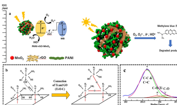
Fig. 27 (a) Schematic illustration of the photocatalytic reduction of MB. Reprinted with permission from ref. 139 Copyright 2019, Elsevier. (b) Illustration of the mechanism of TiO 2 on the surface of GO sheet. (c) XPS spectra of TiO 2 -graphene. Reprinted with permission from ref. 140 Copyright 2020, Elsevier.
