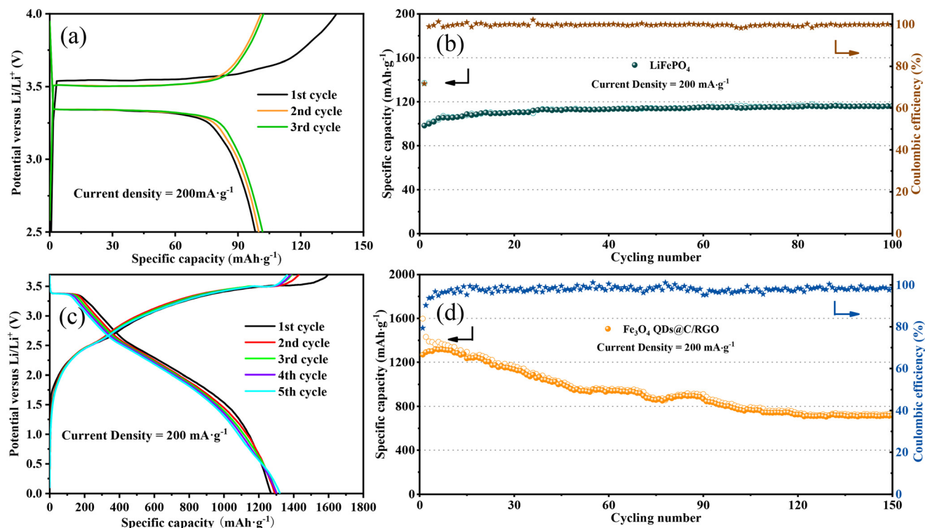
Fig. 8 Charge and discharge voltage profile (a) and cycling performance (b) of a commercial \text{LiFePO}_4 cathode at 200\text{ mA}\cdot\text{g}^{-1} in half cells. Charge and discharge voltage profile (c) and cycling performance (d) of the \text{Fe}_3\text{O}_4 QDs@C/RGO sample in \text{Fe}_3\text{O}_4 QDs@C/RGO// \text{LiFePO}_4 full cells at 200\text{ mA}\cdot\text{g}^{-1} .
