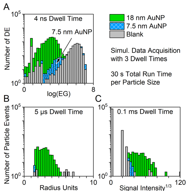
Fig. 8 Comparison of spICP-MS data acquired simultaneously with (A) 4 ns (nanoDAQ), (B) 5 μs (μsDAQ), and (C) 0.1 ms (vendor software) dwell time. Dispersions of AuNP with nominal sizes of 18 and 7.5 nm and a blank solution were measured for 30 s, respectively. Please note that the background signal of nanoDAQ data is on the right side (high log(EG)), while the background in plots from conventional spICP-MS is on the left.
