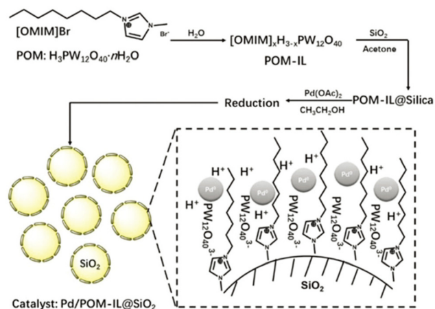
Fig. 8 Schematic illustration of the process for the synthesis of multifunctional catalyst \text{Pd}/\text{POM-IL@SiO}_2 ( \text{Pd}/\text{H}_x[\text{OMIM}]_{3-x}\text{PW}_{12}\text{O}_{40}\text{@SiO}_2 , x = 1, 2, 3 ) and its structure. Adapted from ref. 150 with permission from Royal Society of Chemistry, copyright 2018.
