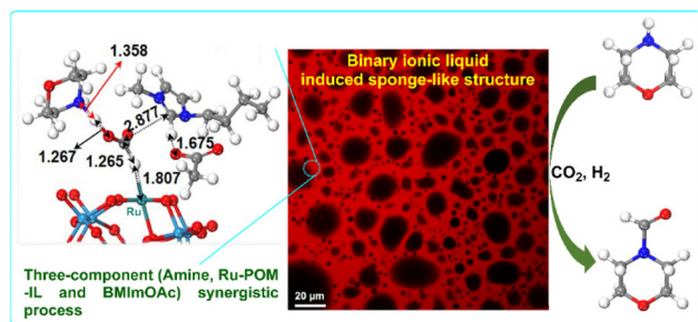
Fig. 7 Ruthenium single-atom anchored in POM–ILs for N -formylation of amines with \text{CO}_2 and \text{H}_2 . Adapted from ref. 89 with permission from American Chemical Society, copyright 2023.
