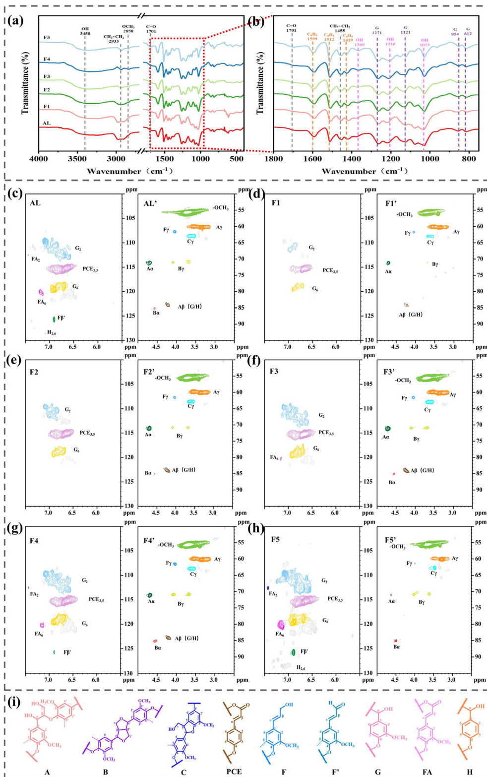
Fig. 1 FTIR spectra of AL and F1–F5 (a); localized enlargement of the FTIR spectra (b). 2D-HSQC NMR spectra of AL and F1–F5 samples (c–h). Main substructures identified in lignin samples (i), A: β-O-4' substructures; B: β-β' resinol substructures; C: phenylcoumaran substructures; PCE: p -coumarate; F: p -hydroxycinnamyl alcohol end groups; F': terminal group structure of hydroxycinnamaldehyde; G: guaiacyl units; FA: ferulate; H: p -hydroxyphenyl units.
