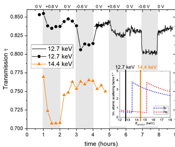
Fig. 1 Measured X-ray transmission as a function of time, obtained at photon energies of 12.7 keV (black full line and black circles) and 14.4 keV (orange triangular symbols). The inset shows the progression of the imaginary part of the atomic scattering factor f'' as a function of the X-ray energies for Rb and Br, with the inset data taken from ref. 24.
