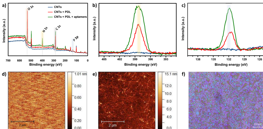
Fig. 2 (a) Wide X-ray spectroscopy (XPS) spectra for bare carbon nanotubes (CNTs) (blue), poly-D-llysine (PDL)-coated CNTs (red), and aptamer-modified CNTs (green). Zoom-in of the (b) N 1s peak intensities (yellow highlight) and (c) P 2p peak intensities (blue highlight) that demonstrate the effective layer-by-layer assembly of PDL and aptamers on the CNTs. (d) Representative atomic force microscopy (AFM) image of the bare waveguide and (e) waveguide coated with spray-deposited CNTs. Increased roughness and height indicate coating of substrates with CNTs. (f) Optical microscopy image of the spray-deposited CNTs-carboxymethyl cellulose surfactant ink on the waveguide. The deposited droplets are close to one another and homogeneously cover the waveguide surface indicative of a high quality surface coating.
