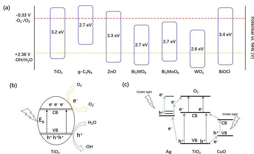
Fig. 5 The mechanism of light-induced reactive oxygen species by semiconductor photocatalysts. (a) Bandgaps of some typical semiconductors. Charge separation of (b) \text{TiO}_2 and (c) Cu and Ag doped \text{TiO}_2 .
