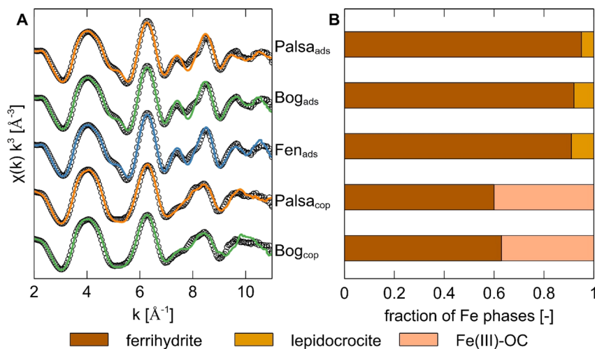
Fig. 2 (A) Iron K-edge k^3 -weighted EXAFS spectra and linear combination fits (2 to 11 \text{\AA}^{-1} ) of ferrihydrite with adsorbed WEOM (ads) from palsa, bog and fen, and Fe-OC coprecipitates (cop) synthesized with WEOM from palsa and bog. Experimental data is displayed as coloured lines and linear combination fits as black circles (see fit parameters in Table S6†). (B) Bar plot showing relative abundances of different Fe phases in the post-adsorption and post-coprecipitation mineral phases. The same labelling as for graph (A) applies here. Fe(III)-OC was fit using Fe(III)-citrate as a reference.
