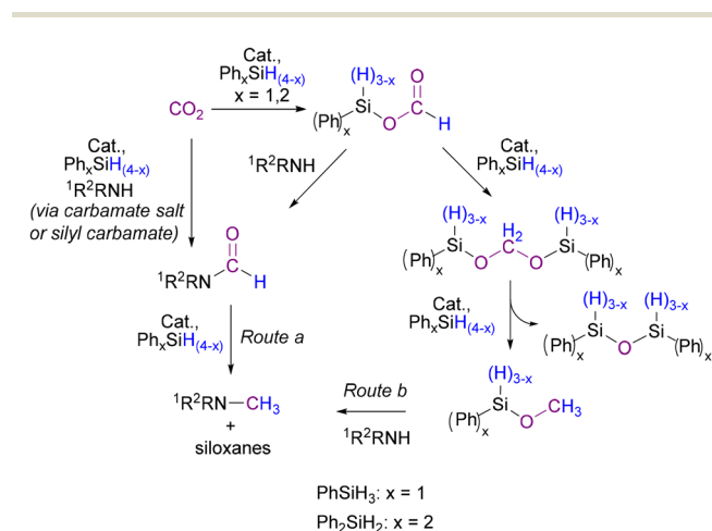
Scheme 7 Supposed reaction routes involved in the N -formylation and N -methylation of amines with \text{CO}_2 and hydrosilanes according to the literature. 56,57,94–97
