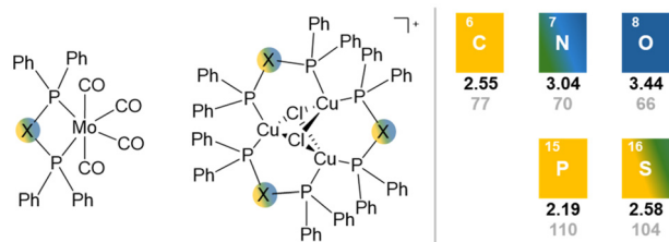
Fig. 6 Comparison of different bridging atoms (C, N, O, S) within the backbone of short-bite diphosphine ligands using [Mo(CO) 4 (PXP)] and the cation [Cu 3 (μ 3 -Cl) 2 (μ-PXP) 3 ] + as examples. The electronegativity of the respective element is given in black and the covalent radii [pm] is given in grey (right). The hard/soft character of the bridging atoms are displayed by colours: yellow: soft, green: intermediate, blue: hard.
