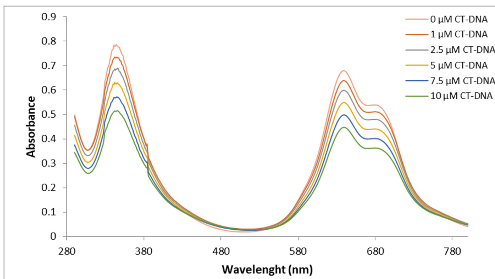
Fig. 2 Absorption titration spectra of ZnPc-2 in Tris-HCl buffer with increasing amounts of CT-DNA.
