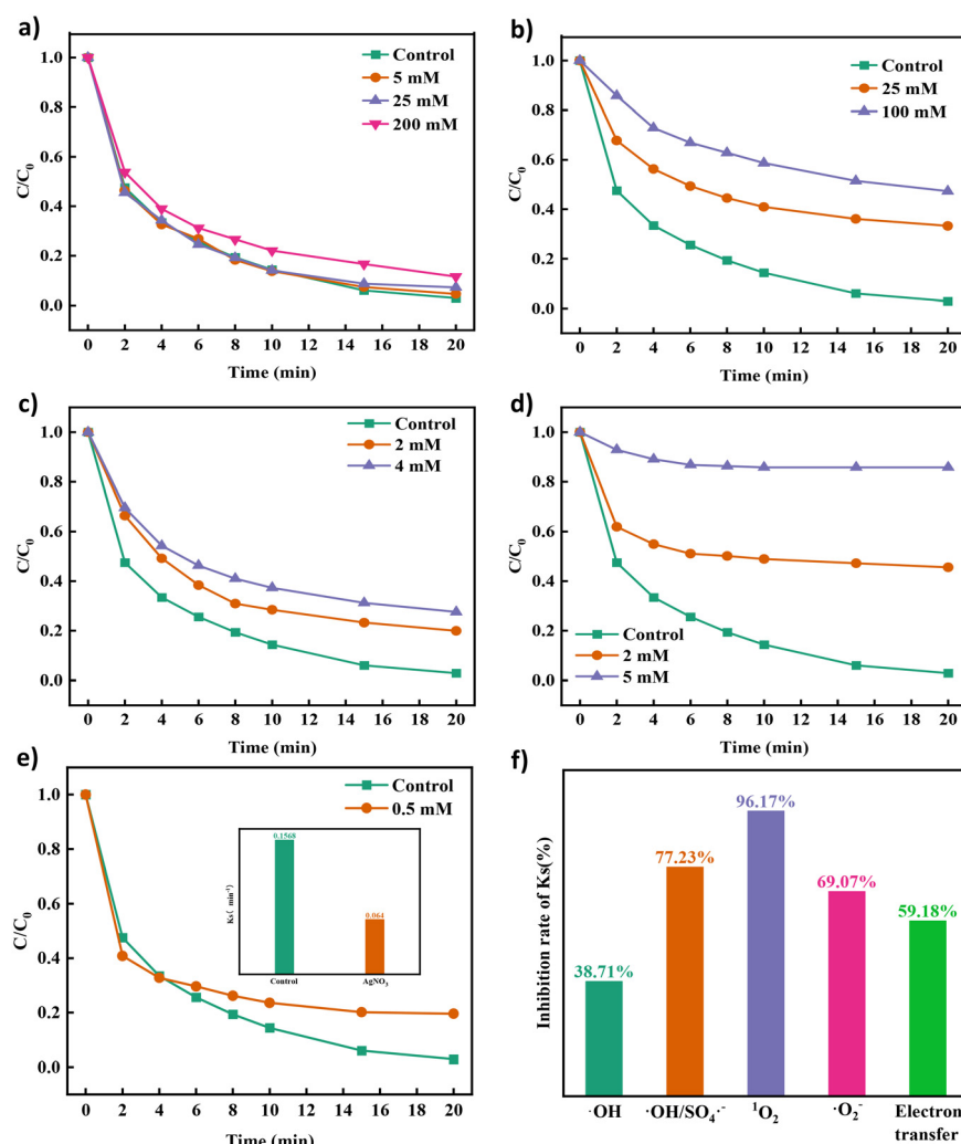
Fig. 3 Effect of different quenching agents TC, (a) TBA, (b) MeOH, (c) p -BQ, (d) L-his and (e) different concentrations of silver nitrate on the degradation efficiency of TCH and (f) the change in its first-order reaction kinetic coefficient.
