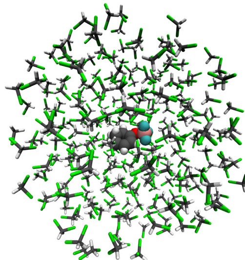
Fig. 1 Equilibrated cyclohexenone-BF 3 complex in DCM.
