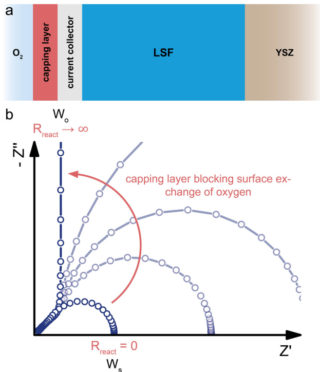
Fig. 7 (a) Schematic sketch of a dense SOFC electrode consisting of a predominant electronic conductor (LSF, \sigma_{ion} \ll \sigma_{eon} ) on a YSZ electrolyte contacted by a current collector on the O_2 -exposed side. A capping layer blocks the surface exchange reaction between the O_2 atmosphere and the LSF surface. (b) Evolution of the calculated impedance response (circuit Fig. 6b with R_{eon} = 0 ) for an increasing surface exchange resistance R_{react} due to the capping layer, showing the gradual transition from a W_s to a W_o type behavior.
