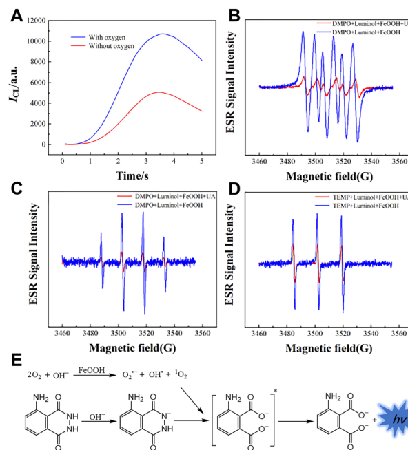
Fig. 12 (A) CL kinetic curves of the luminol/FeOOH system in the absence and presence of oxygen. ESR spectra of adducts. (B) DMPO–O 2 * - (C) DMPO–OH* - and (D) TEMP– 1 O 2 in the luminol/FeOOH CL system. (E) Mechanism of the luminol/FeOOH CL system. [Luminol]: 100 μM; [FeOOH]: 25 μg mL -1 ; [UA]: 5 μM; [pH]: 10.0. Reprinted with permission from ref. 63, Copyright 2023 American Chemical Society.
