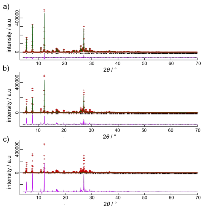
Figure 2. Results of Rietveld refinement against experimentally measured PXRD pattern for a sample of caf-pyg-4H 2 O : a) herein determined single crystal structure of caf-pyg-4H 2 O ; b) the best simulated annealing PXRD structure solution and c) the caf-pyg-5H 2 O structural model after DFT optimisation (see also ESI).
