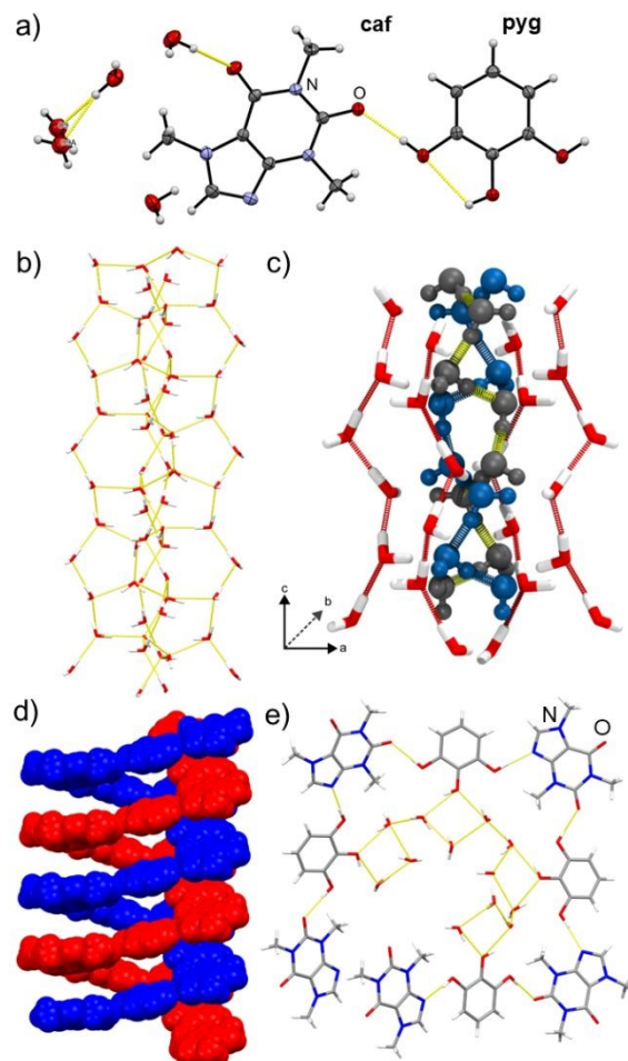
Figure 1. a) ORTEP view of the asymmetric unit of caf-pyg ·4H 2 O, with non-hydrogen atoms shown as ellipsoids of 50% probability. Views of the crystal structure of caf-pyg ·4H 2 O: b) a single hydrogen-bonded column; c) two disordered core chains, shown in ball-and-stick style and colored blue and black, surrounded by an envelope of water molecules shown in stick style; d) two interwoven hydrogen-bonded caf-pyg helices and e) repeat unit of a caf-pyg helix viewed along the crystallographic c -axis.
