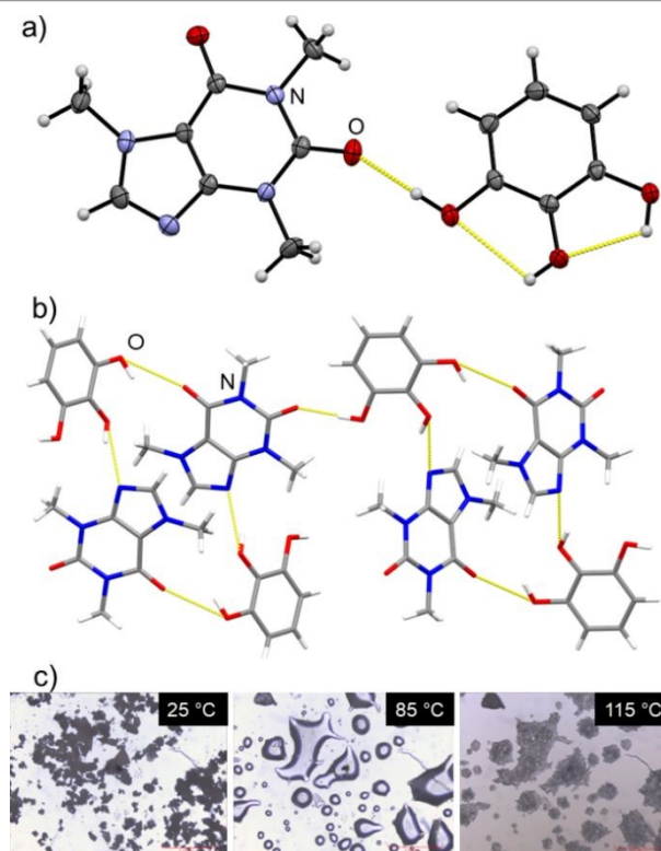
Figure 3. a) ORTEP representation of the asymmetric unit of caf-pyg , with non-hydrogen atoms show as 50% probability ellipsoids; b) view of the caf-pyg crystal structure, illustrating the hydrogen-bonded assembly of molecules; c) hot-stage microscopy images of caf-pyg-4H 2 O , illustrating the liquefaction and recrystallisation (also see ESI).
