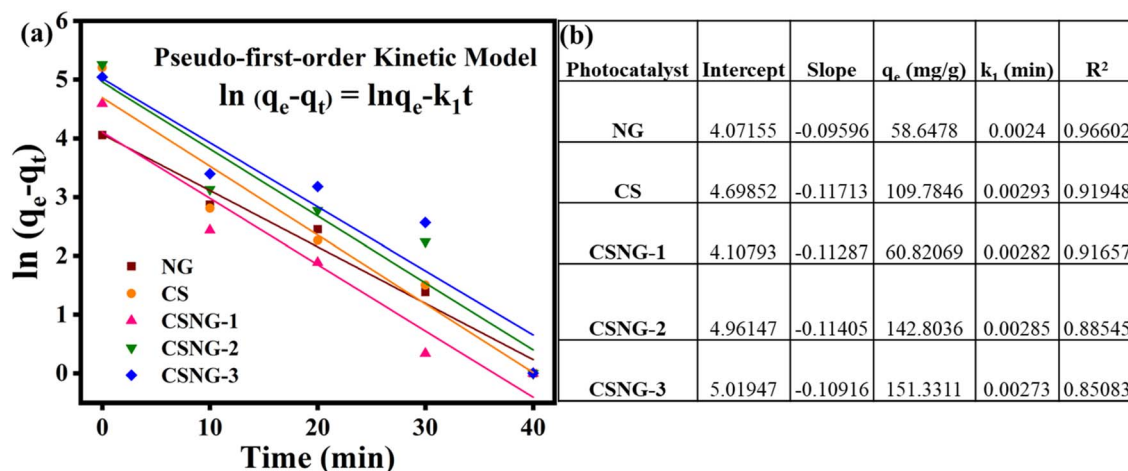
Fig. 8 (a and b) The pseudo-first-order-kinetic model with time.
