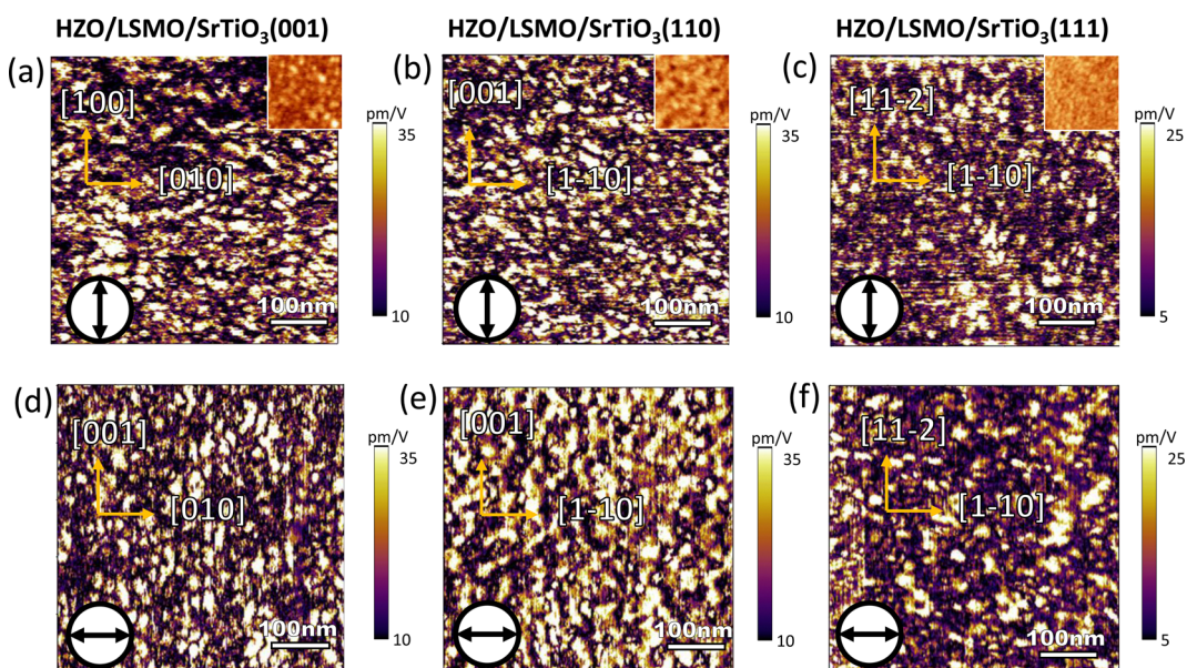
Fig. 5 (a–c) PFM in-plane amplitude images for the HZO films on LSMO/SrTiO 3 (001), LSMO/SrTiO 3 (110) and LSMO/SrTiO 3 (111), respectively. Response is probed along the vertical direction as indicated in the bottom-left. Top-right insets show the topography images. (d–f) Idem, while probing along the horizontal direction.
