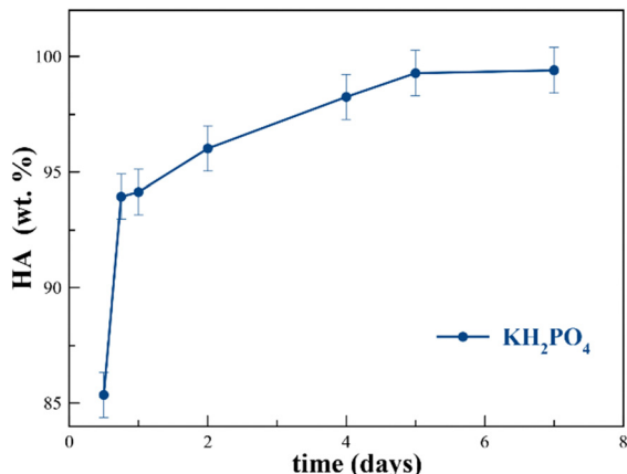
Fig. 2 Evolution of HA wt% with time using KH 2 PO 4 at a P/bCCP molar ratio 0.6.
