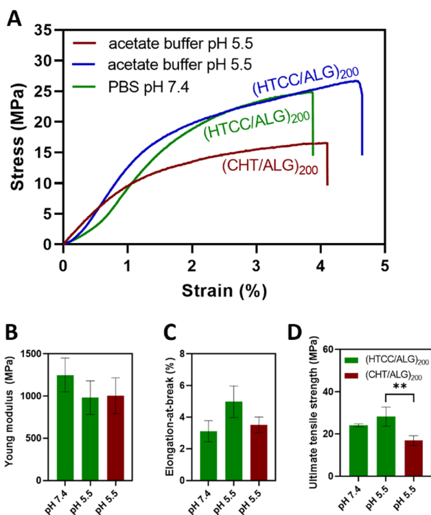
Fig. 8 Mechanical properties of the FS membranes in PBS (pH 7.4) and acetate buffer (pH 5.5). (A) Representative stress-strain curves, (B) Young modulus, (C) elongation-at-break, and (D) ultimate tensile strength. Data are presented as mean \pm SD of three independent experiments ( n = 3 , per condition) performed in triplicates. Significant differences were found for ** p \leq 0.01 .
