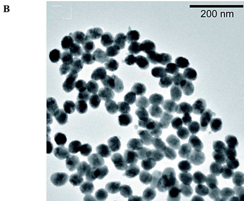
Fig. 5 (A) The preparative process of the Au nanostructures using a surfactant-free electrodeposition method. The porous anodic alumina template was treated by pore widening or barrier layer thinning, after the two-step anodization procedure; the nanostructures were branched or round-bottomed, respectively. (B) TEM image of Au NPs produced using a templated and surfactant-free electrodeposition approach (time: 100 s). Adapted from ref. 84 with permission. Copyright 2022 Royal Society of Chemistry (CC BY).
