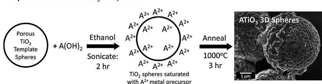
Fig. 4 The preparative process of ATiO 3 micron-scale spheres. Adapted from ref. 77 with permission. Copyright 2021 Multidisciplinary Digital Publishing Institute (CC BY).
