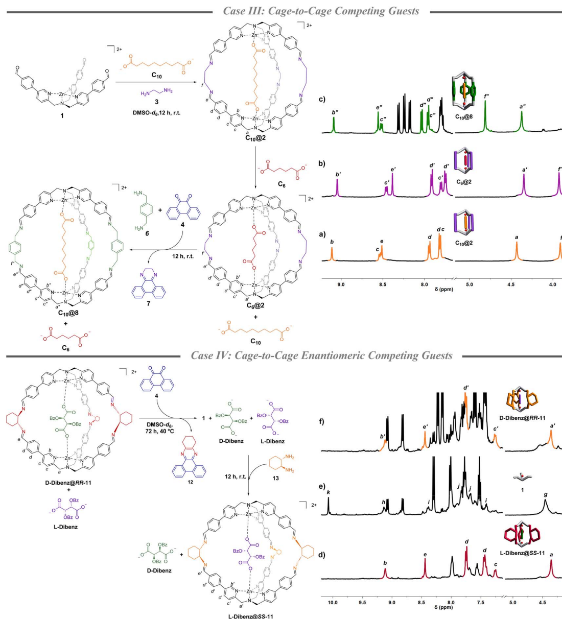
Fig. 2 Case III: partial ^1\text{H} -NMR ( \text{DMSO}-d_6 , 500 MHz) of (a) \text{C}_{10}@2 , (b) \text{C}_6@2 obtained after the complete exchange of the guest, and (c) \text{C}_{10}@8 obtained after the addition of quinone 4 and p -xylylenediamine 6 to the mixture of \text{C}_6@2 and \text{C}_{10} . p -Xylene is used as the internal standard. Case IV: partial ^1\text{H} -NMR ( \text{DMSO}-d_6 , 400 MHz) of (d) D-Dibenz@RR-11 (d.r. 17 : 1 between the two guests), (e) complex 1 obtained from cage disassembly using quinone 4 , and (f) 12 h after the addition of S,S -diaminocyclohexane 13 that led to the formation of L-Dibenz@SS-11 and the exchange in the selectivity for the two guests. 1,3,5-Trimethoxybenzene is used as the internal standard.
