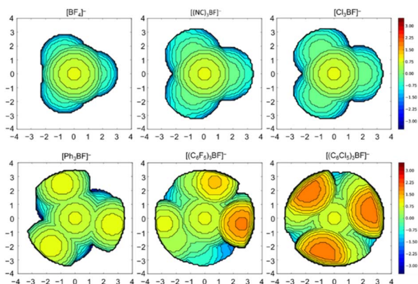
Fig. 2 Topographic steric maps of the Lewis acids BF 3 , B(CN) 3 , BCl 3 , BPh 3 , B(C 6 F 5 ) 3 , and B(C 6 Cl 5 ) 3 in their fluoride adducts [BF_4]^- , [(NC)_3BF]^- (MFB), [Cl_3BF]^- , [Ph_3BF]^- , [(C_6F_5)_3BF]^- , and [(C_6Cl_5)_3BF]^- ( d(B-F) = 1.40 Å and R = 3.50 Å). The isocontour scheme is given in Å, red and blue zones indicate the more- and less-hindered zones with respect of the origin.
