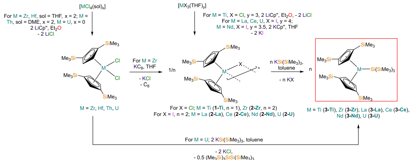
Scheme 1 Synthetic routes to complexes 3-M.
