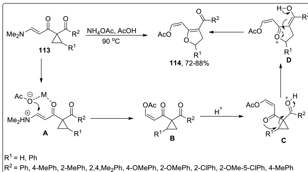
Scheme 35 Synthesis of substituted dihydrofurans 114 via Cloke–Wilson rearrangement.
