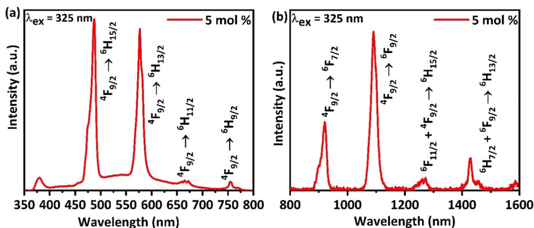
Fig. 7 (a) Emission spectra of \text{Ba}(\text{La}_{2-x}\text{Dy}_x)\text{ZnO}_5 ( x = 5 \text{ mol \%} ) from UV to visible and (b) visible to NIR regions of the electromagnetic spectrum recorded by using an excitation wavelength of 325 nm.
