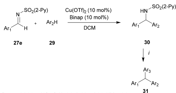
Scheme 7 One-pot synthesis of unsymmetrical triarylmethanes through a copper-catalyzed aza-FC reaction. R = p -tolyl ( a ), p - \text{NO}_2 - \text{C}_6\text{H}_4 ( b ), 2-thienyl ( c ), \text{NMe}_2 ( d ) \text{Ar}_1, \text{Ar}_2, \text{Ar}_3 = indolyl, (5-OMe)- N -methylindolyl, 2,4,6-triOMePh, 2-OMe-thiophenyl... i : if \text{Ar}_2 = indolyl: \text{Ar}_3\text{H} , 40°C (one-pot); for other aromatic groups: \text{Ar}_3\text{H} , \text{Sc}(\text{OTf})_3 10 mol%, ACN, 60°C
