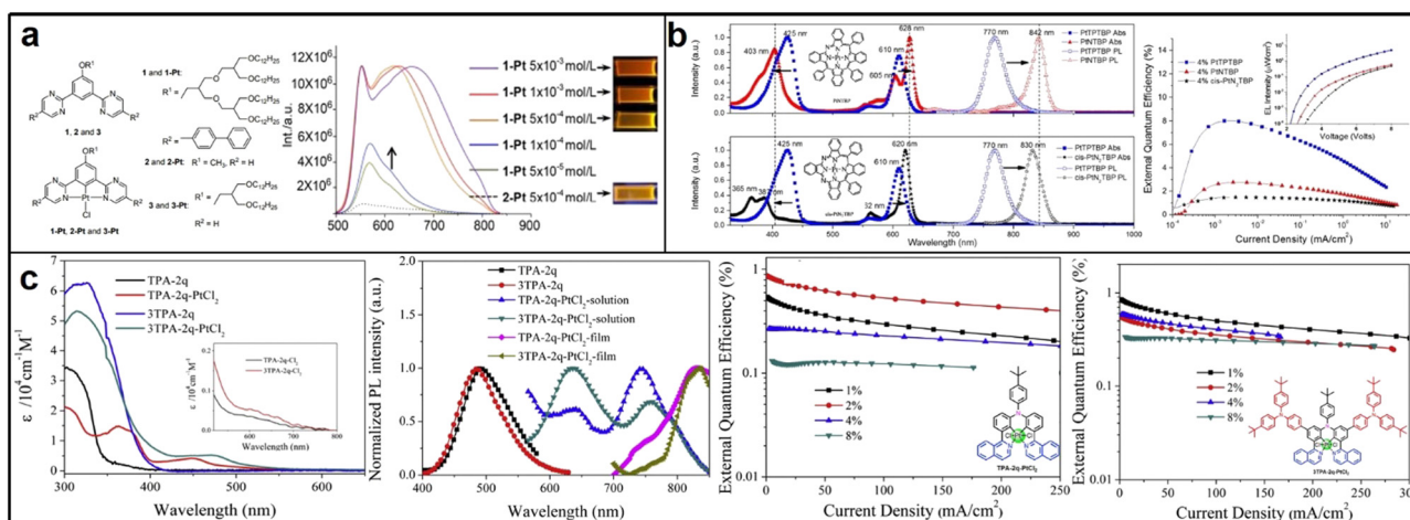
Fig. 6 (a) N ^C^N -type tridentate ligand-based Pt(II) complexes; reproduced with permission from ref. 59. Copyright 2017 Chinese Journal of Organic Chemistry . (b) PtNTBP and cis -PtN₂TBP; reproduced with permission from ref. 61. Copyright 2016 Applied Physics Letters . (c) TPA-2q-PtCl₂ and 3TPA-2q-PtCl₂. Reproduced with permission from ref. 62. Copyright 2017 Dyes and Pigments .
