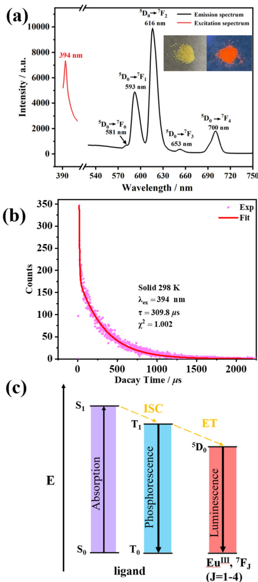
Fig. 5 (a) Excitation and emission spectra; (b) luminescence lifetime; and (c) Jablonski level diagrams of \text{Eu}_{28} .
