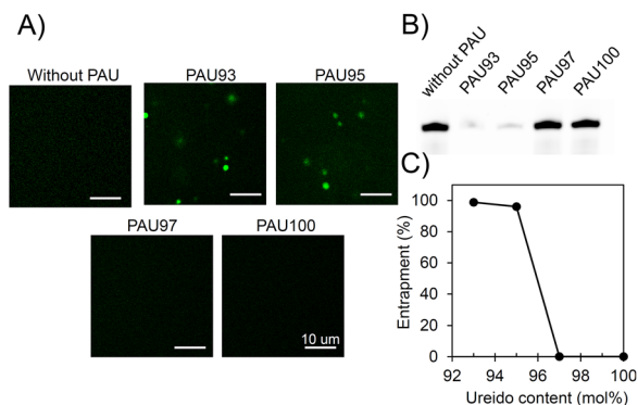
Fig. 3 (A) Microscopic images of 100 \text{ nM} FITC-labelled DNAzyme in the presence of 1 \text{ mg mL}^{-1} PAUs at 35 \text{ °C} . Scale bars indicate 10 \text{ }\mu\text{m} . (B) PAGE analysis of supernatants prepared from FITC-labelled DNAzyme alone or DNAzyme in the presence of PAUs. (C) Percent entrapped DNAzyme as a function of ureido content of PAU.
