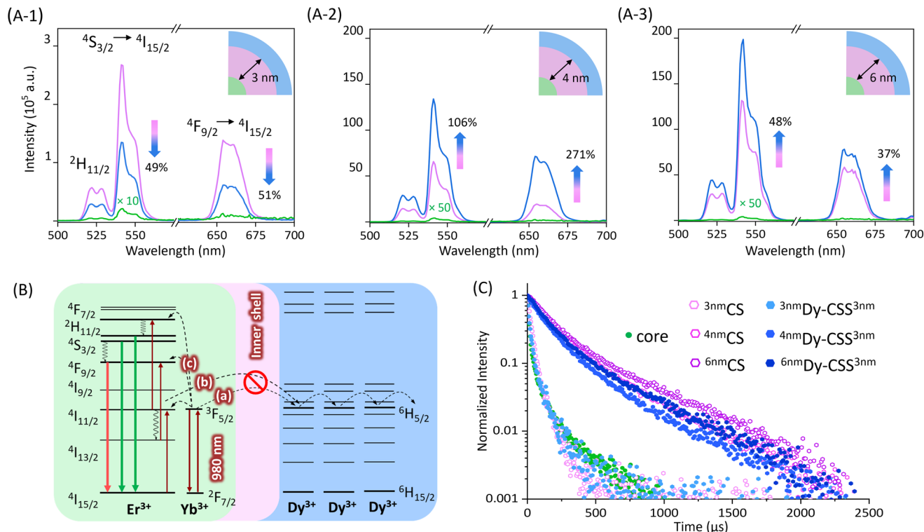
Fig. 2 (A) UC spectra of OA-capped ^3\text{nmDy-CSS}^3\text{nm} (1), ^4\text{nmDy-CSS}^3\text{nm} (2), and ^6\text{nmDy-CSS}^3\text{nm} (3) NPs (blue) as well as their corresponding core (green) and CS (pink) NPs. All spectra were obtained under 980 nm laser excitation. Power density = 6.0 \text{ W cm}^{-2} , [\text{NP}] = 5 \text{ mg mL}^{-1} in toluene. (B) Partial energy level diagram for \text{Er}^{3+}/\text{Yb}^{3+} and \text{Dy}^{3+} , schematically showing how the addition of an inner shell physically separates \text{Er}^{3+}/\text{Yb}^{3+} from \text{Dy}^{3+} ions, thus, preventing \text{Dy}^{3+} -induced loss of the UC. Solid lines are radiative transitions, dotted lines indicate energy transfer, and wavy lines are non-radiative transitions. (C) Luminescence decay curves of the \text{Yb}^{3+} emission under 980 nm excitation obtained from core, CS, and CSS NPs.
