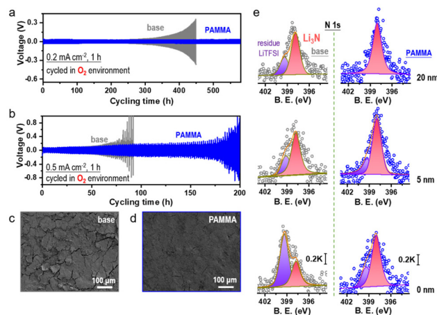
Fig. 2 Electrochemical performance of Li/Li symmetrical cells under O 2 environment without (gray trace)/with PAMMA (blue trace) at current densities of (a) 0.2 mA cm -2 and (b) 0.5 mA cm -2 . Surface morphology characterization of the cycled Li-metal in the Li/Li symmetrical cell under O 2 atmosphere (c) without and (d) with PAMMA (after 50 cycles, 0.2 mA cm -2 , 1 h). (e) N 1s spectra of the cycled Li-metal surface without/with PAMMA in Li/Li symmetrical cell at different etching depths of 0, 5, and 20 nm (O 2 atmosphere, after 50 cycles, 0.2 mA cm -2 , 1 h).
