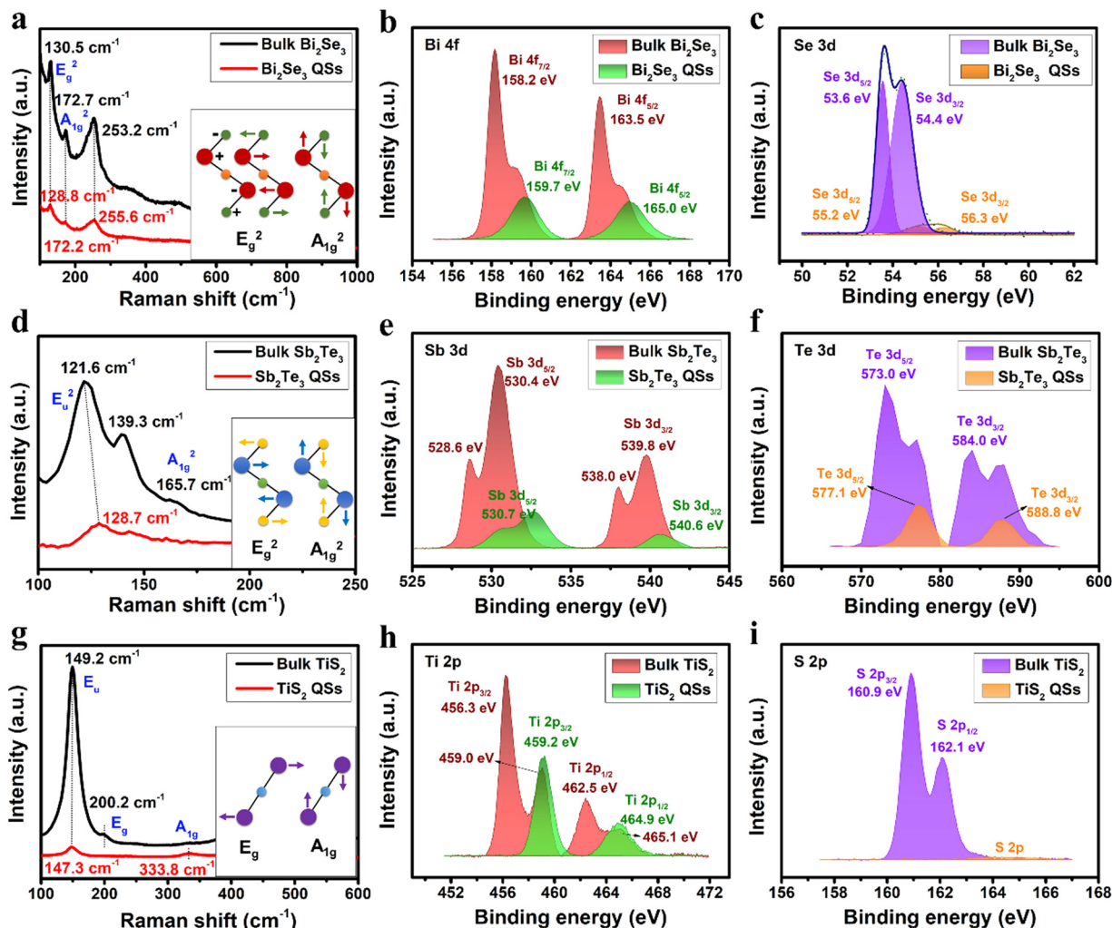
Fig. 2 Spectroscopic characterization of the as-produced QSSs. Raman spectra of (a) Bi 2 Se 3 QSSs, (d) Sb 2 Te 3 QSSs, and (g) TiS 2 QSSs. High-resolution XPS spectra of (b), (c) Bi 2 Se 3 QSSs, (e), (f) Sb 2 Te 3 QSSs, and (h), (i) TiS 2 QSSs. Data for bulk materials are shown for comparison.
