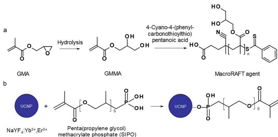
Fig. 1 (a) Preparation of poly(glycerol methacrylate)-based macroRAFT agent and (b) surface modification of UCNP with SIPO.
