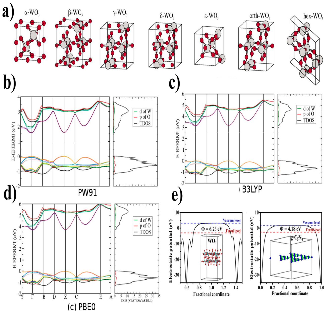
Fig. 5 (a) The unit cells of \text{WO}_3 at different temperatures show different phases (reproduced with permission from ref. 79 Copyright 2010, AIP Publishing). (b) PW91, (c) B3LYP, (d) PBE0 (band structure and density of states (DOS) of room-temperature monoclinic \text{WO}_3 by different kinds of functionals) (reproduced with permission from ref. 81 Copyright 2011, American Chemical Society). (e) Electrostatic potentials \text{WO}_3 (001) surface and g\text{-C}_3\text{N}_4 (001) surface (reproduced with permission from ref. 82 Copyright 2018, Elsevier).
