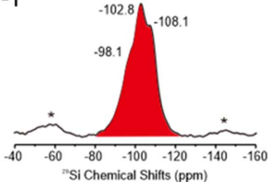
Fig. 2 ^{29}\text{Si} NMR spectra of unsubstituted and N-substituted ZSM-5, \beta , and Y zeolites, referenced to Kaolin ( -91.5 ppm).
