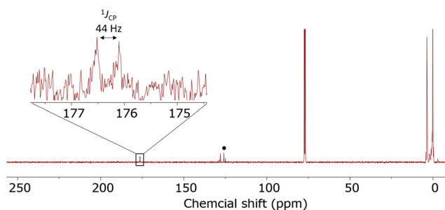
Fig. 8 ^{13}\text{C}\{^1\text{H}\} NMR spectra for the reaction of (\text{Me}_3\text{Si})_3\text{P}_7 with \text{CO}_2 . Dissolved \text{CO}_2 marked with \bullet .
