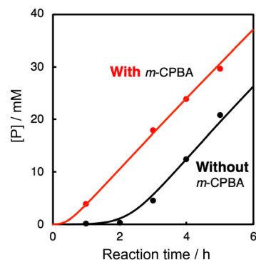
Fig. 4 Time courses of the cyclohexane oxidation by the O 2 /1/PhCHO system with and without m -CPBA (10 mM). Reaction conditions: [1] = 0.025 mM, [PhCHO] = 0.2 M, [cyclohexane] = 2.0 M at 40 °C under O 2 .
