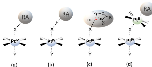
Scheme 3 Inner-sphere mechanisms for the reduction of Pt IV complexes by a generic reducing agent (RA) or a specific one (AscH - ). (a) Ligand-bridge electron transfer; (b) ligand-bridge-H transfer; (c) enolate \beta -carbon attack; (d) Pt(II)-catalysed mechanisms.
