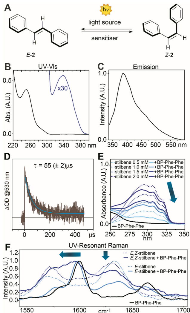
Fig. 3 (A) Photoisomerisation of E -stilbene (E-2). (B) UV-Vis spectra of BP-Phe-Phe. (C) BP-Phe-Phe emission spectrum (ex. 315 nm). (D) BP-Phe-Phe triplet state lifetime. (E) UV-Vis spectra of stilbene without and with BP-Phe-Phe (1 mM, cac). (F) UVR spectra of BP-Phe-Phe, stilbene, and their mixtures, all in MeCN.
