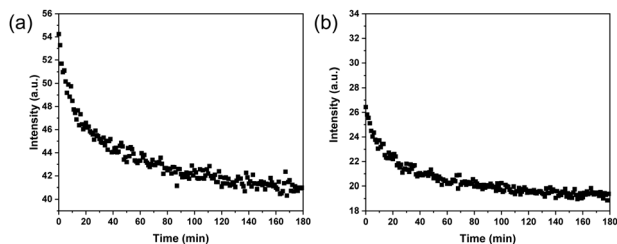
Fig. 4 (a) Change in fluorescence intensity of ARS-loaded MIP particles ( 0.5 \text{ mg mL}^{-1} ) measured after the addition of 1 M fructose. (b) Change in fluorescence intensity of ARS-loaded NIP particles ( 0.5 \text{ mg mL}^{-1} ) measured after the addition of 1 M fructose. The fluorescence intensity was measured at 560 nm in 20 mM phosphate buffer.
