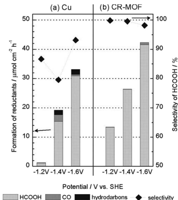
Fig. 8 Contrast between the electrocatalytic performance and selectivity of Hinogami et al. (ref. 100). Cu–rubeanic acid MOF and a Cu electrode (ref. 100, ©The Electrochemical Society. Reproduced by permission of IOP Publishing Ltd all rights reserved).
