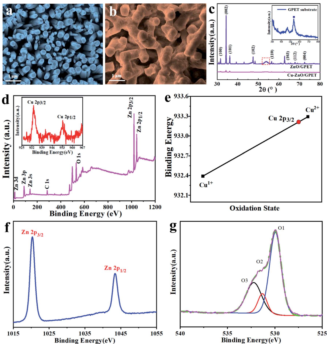
Fig. 1 The FESEM images of (a) ZnO/GPET and (b) \text{Cu}_1 -ZnO/GPET. (c) The XRD patterns of ZnO/GPET and \text{Cu}_1 -ZnO/GPET nanomaterials, where inset shows GPET substrate peaks. (d) XPS spectra for \text{Cu}_1 -ZnO/GPET films and the inset shows Cu 2p peaks. (e) The binding energy of Cu 2p_{3/2} with +2 and +1 oxidation states, respectively. (f and g) High resolution XPS scan of Zn 2p and O 1s for \text{Cu}_1 -ZnO/GPET.
