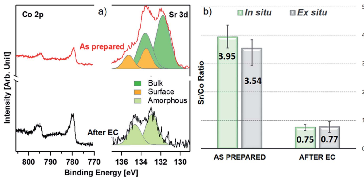
Fig. 2 Photoemission spectra (a) acquired at h\nu = 2300 eV during the in situ experiment showing the collapse of the Sr 3d signal peak (right) compared to the Co 2p signal (left) with red and black curves corresponding to the "as prepared" and "after electrochemistry" state, respectively. The dark green component of the strontium deconvolution corresponds to the bulk signal, orange corresponds to the surface signal, and the light green single component seen after electrochemistry corresponds to the new single species displaying a shift in the binding energy. The Sr/Co ratios calculated from these spectra are shown as histograms (b) with the in situ experiment plotted in light green and the ex situ one plotted in gray.
