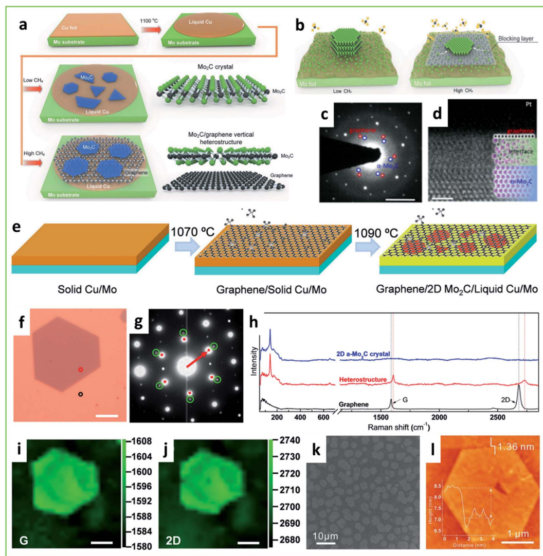
Fig. 2 (a) Schematic illustration of CVD growth of Mo_2C crystals; (b) schematic for growth of Mo_2C and Mo_2C /graphene structures under low and high CH_4 gas flow concentrations; (c) SAED pattern of hexagonal \alpha - Mo_2C /graphene heterostructure (scale bar is 1\ \mu m ), (d) HAADF-STEM images of interfaces; (e) schematic for direct growth of \alpha - Mo_2C /graphene heterostructure through two-step CVD; (f) optical image of \alpha - Mo_2C /graphene heterostructure showing compressed graphene; (g) SAED pattern of 2D \alpha - Mo_2C region; (h) Raman spectra of pure \alpha - Mo_2C , graphene and \alpha - Mo_2C /graphene heterostructure for the images shown in (f) (red circle indicates heterostructure); (i and j) G and 2D peak position mappings of a \alpha - Mo_2C /graphene heterostructure grown using CVD method (scale bar is 5\ \mu m ); (k) SEM image of WC single crystal embedded in graphene; and (l) AFM image of WC single crystal and thickness analysis. (a and b) Are adapted with permission. 74 Copyright 2017, Wiley-VCH, (c and d) is adapted with permission. 78 Copyright 2018, American Physical Society, (e–j) are adapted with permission. 76 Copyright 2017, American Chemical Society, and (k and l) adapted with permission. 68 Copyright 2017, Elsevier.
