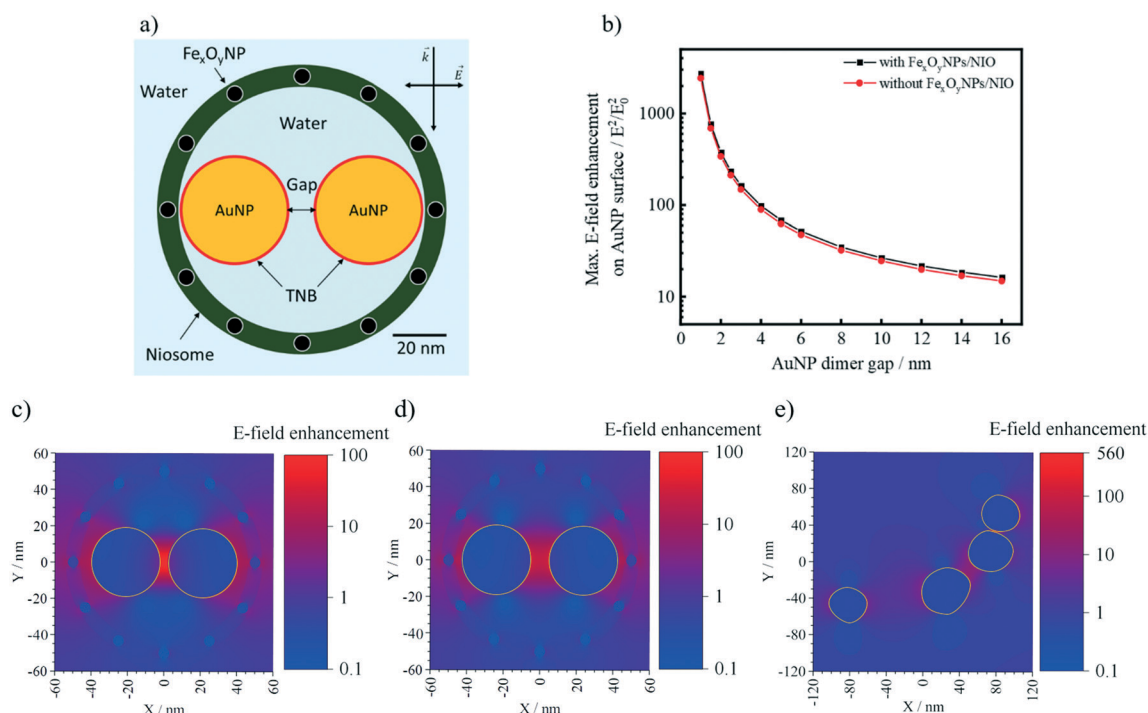
Fig. 6 a) Schematic representation of AuNPs/ \text{Fe}_x\text{O}_y\text{NPs} /NIO utilized for the FDTD simulations; b) calculated maximum E-field enhancement on the AuNP surface for AuNPs/ \text{Fe}_x\text{O}_y\text{NPs} /NIO and AuNPs/NIO with variant interparticle gap; FDTD simulated E-field enhancement of AuNPs/ \text{Fe}_x\text{O}_y\text{NPs} /NIO with a AuNP (encircled in gold) gap distance of c) 4 nm, d) 10 nm, and e) for the AuNPs/ \text{Fe}_x\text{O}_y\text{NPs} /NIO from the TEM image in Fig. 5e.
