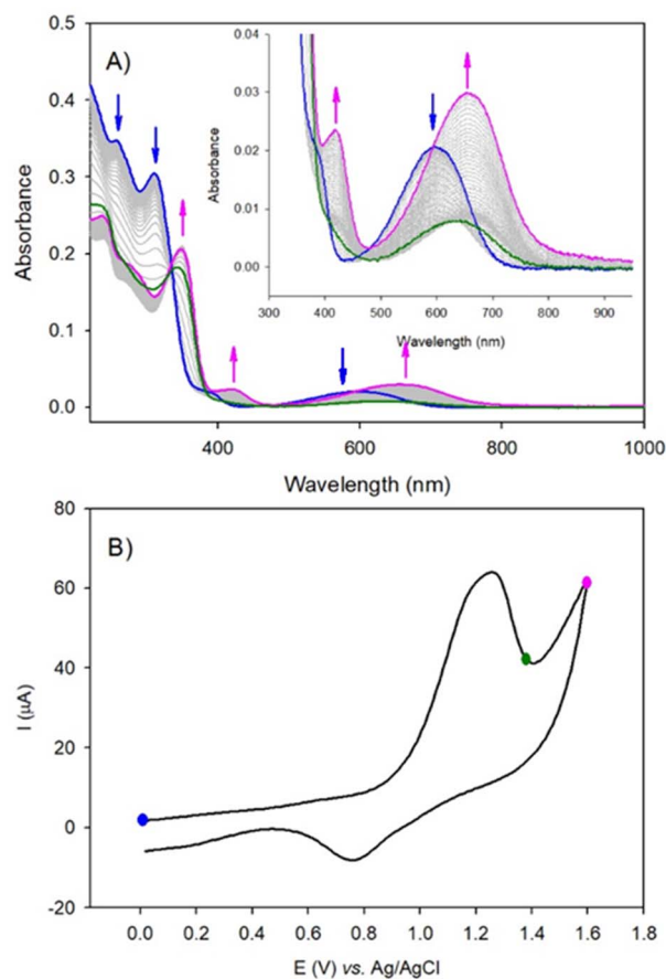
Fig. 6 UV-vis-NIR spectroelectrochemistry of ((1(O_A)_x(C)_z)) , ( c = 1.72 \times 10^{-4} M, 20 °C) upon electrochemical oxidation in 0.1 M n\text{-Bu}_4\text{NPF}_6 in acetonitrile/1,4-dioxane (1/1) solution at a scan rate of 20 \text{ mV s}^{-1} . (A) Evolution of the UV-vis-NIR spectra recorded during oxidation. Optical path length = 0.02 cm. (B) CV at a scan rate of 20 \text{ mV s}^{-1} recorded during the spectroelectrochemistry measurement. Note that the start of the recording (blue curve) is done when the equilibrium from closed to open form is reached under UV-visible illumination.
